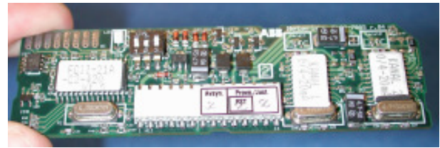
Fig.1, Analog input board, component side
